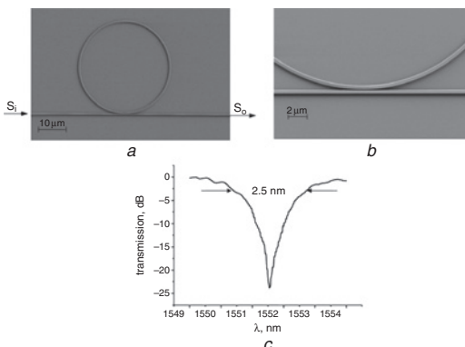
Fig. 1 SEM photo of fabricated single coupled silicon microring resonator (cross-section of silicon waveguide 450 \times 250 \text{ nm}^2 ); zoom-in view of coupling region; measured transmission spectrum of silicon ring resonator
