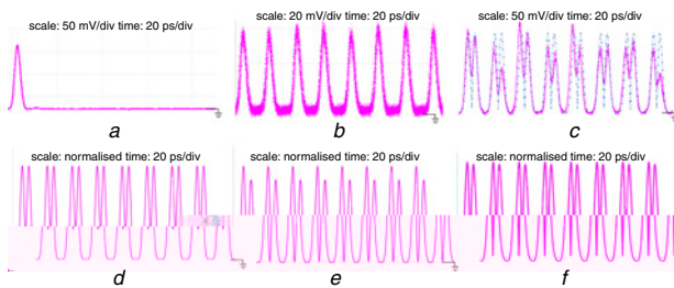
Fig. 3 10 Gbit/s picosecond pulses (Fig. 3a); 80 Gbit/s signals after optical multiplexer (OMUX) (Fig. 3b); measured (solid) and simulated (dotted, ideal differentiation) 80 Gbit/s output OTDM signals after optical differentiation (Fig. 3c); simulated 80 Gbit/s OTDM signals after differentiation considering the limited bandwidth of 500 GHz oscilloscope (bandwidth of 500GHz) (Fig. 3d); simulations of waveforms after silicon ring (Figs. 3a,f) with same parameters in experiment (notch depth of 24 dB and 3 dB bandwidth of 2.5 nm) (Fig. 3e) and notch depth of 30 dB and 3 dB bandwidth of 2.5 nm (Fig. 3f)
